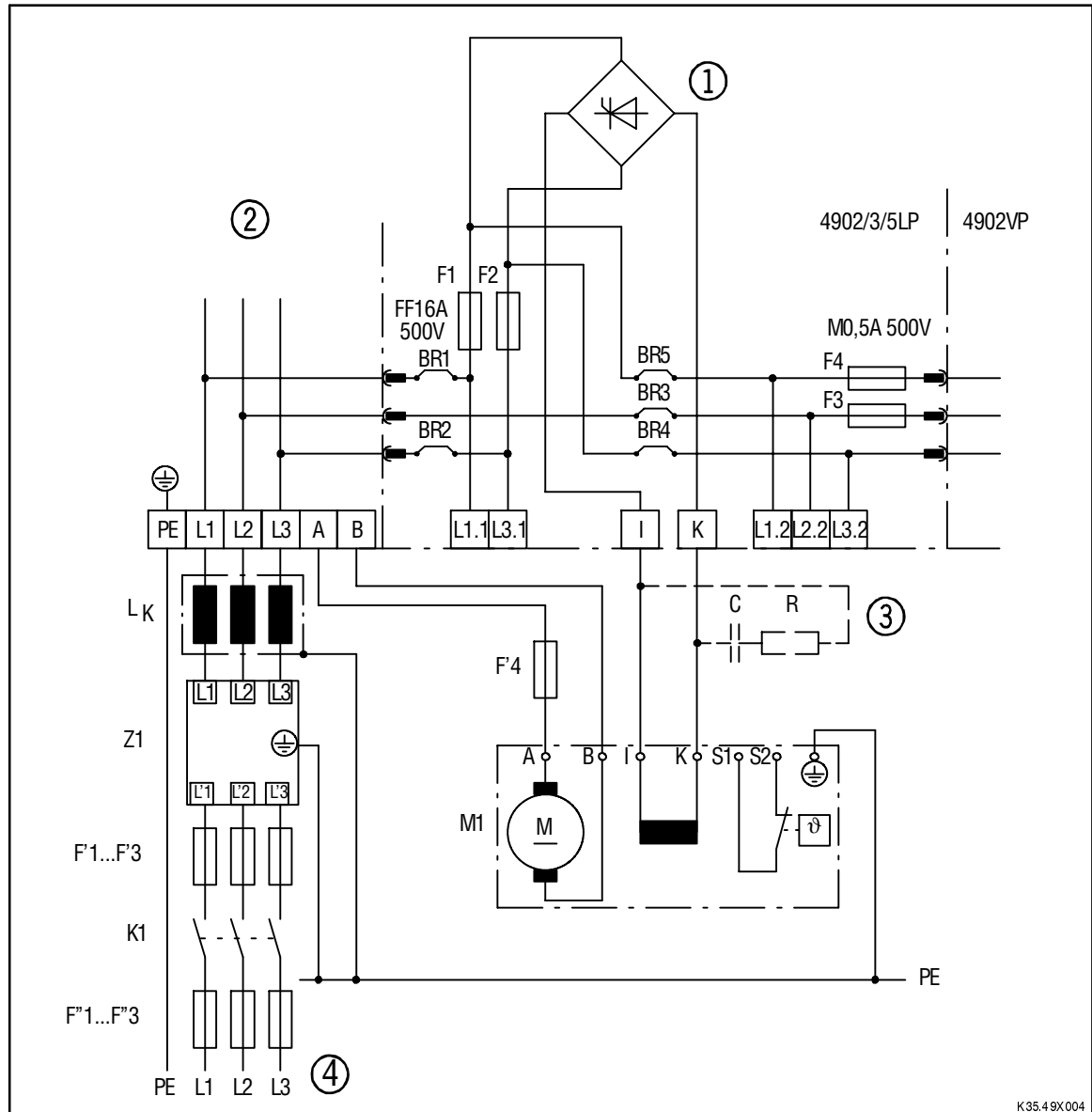
FIG 4-3 Power connection of controllers 4902 to 4907
