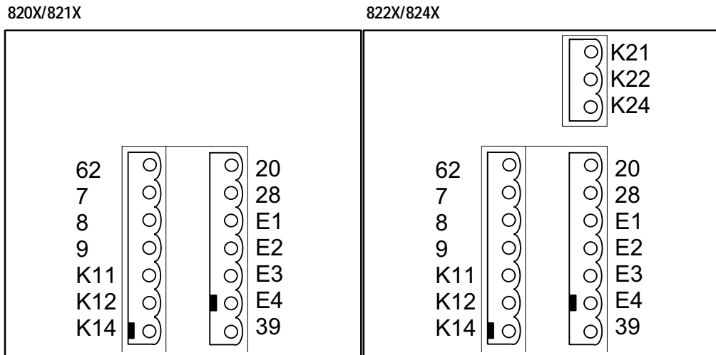
FIG 4-23 Layout of the control terminals
