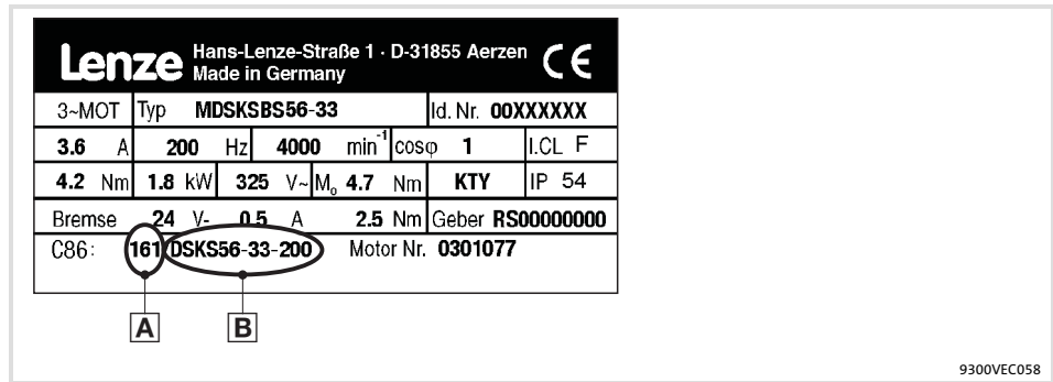
Fig. 6.6-2 Nameplate of a Lenze motor
