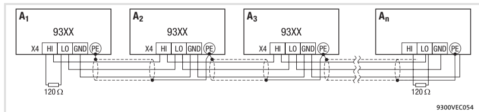
Fig. 5.10-1 System bus (CAN) wiring
