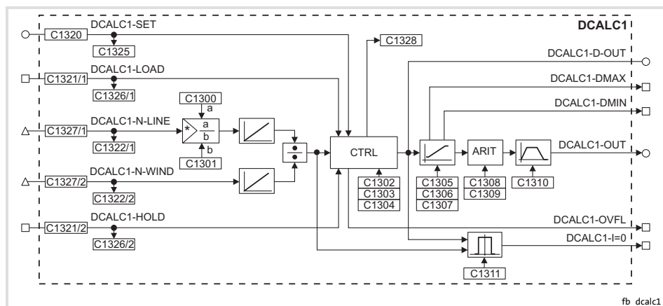
Fig. 8.2-1 Diameter calculator (DCALC1)
