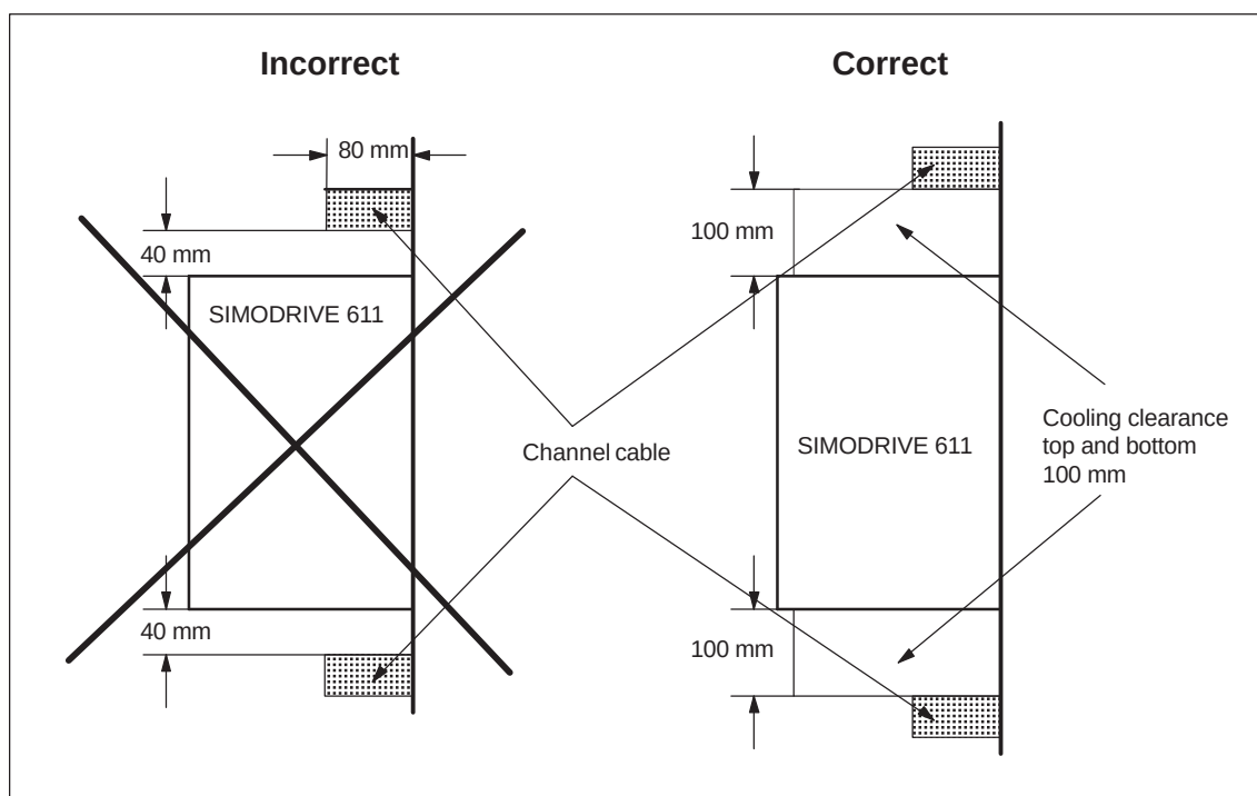
Fig. 9-4 Cooling clearance
